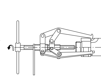
Fig. 14.14 Removal of Inner Ring Using Withdrawal Tool (2)
