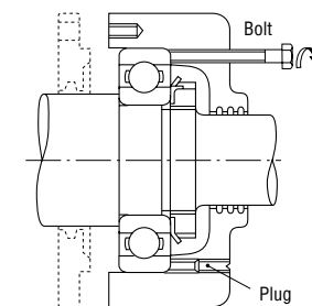
Fig. 14.10 Removal of Outer Ring with Dismounting Bolts
