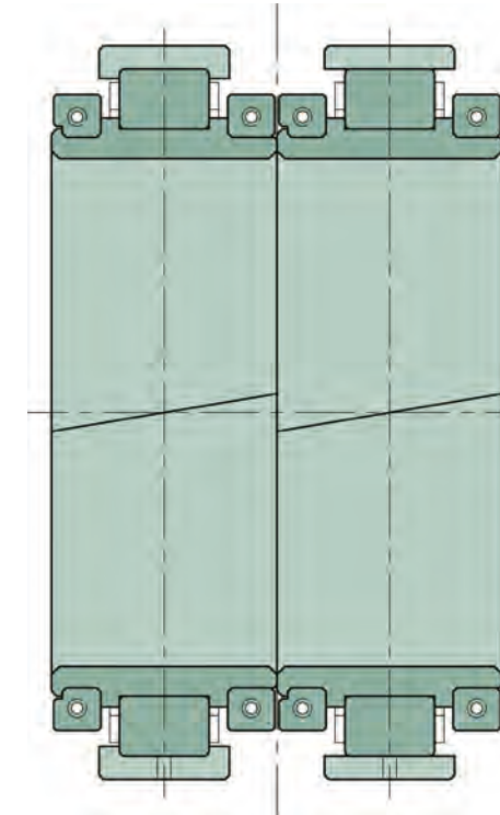
Double Bearings
