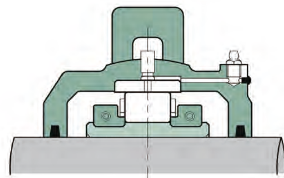
EX Bearing (D Type)
