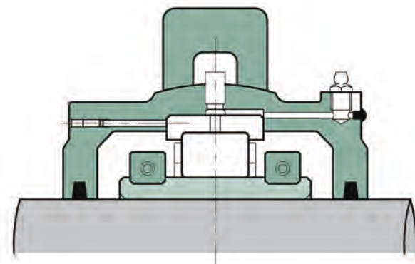
EXILOG Bearing
