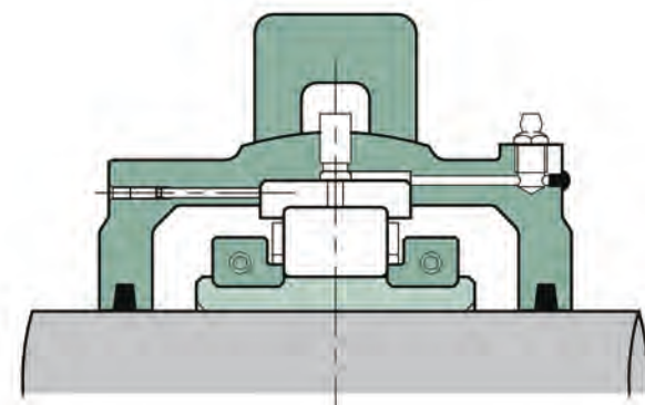
GR Bearing (D Type)
