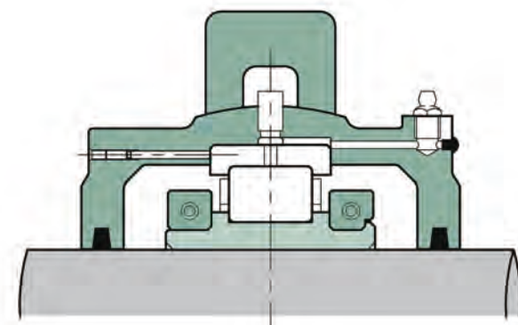
GR Bearing (C Type)
