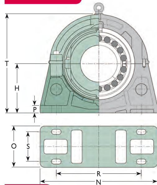
PEDESTAL
