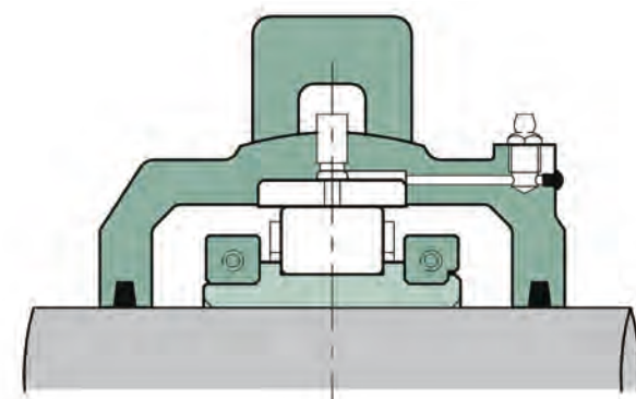
EX Bearing (C Type)
