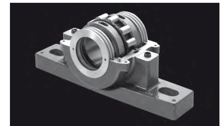
This picture illustrates an aluminium triple labyrinth seal on an OIE Series bearing and cartridge.
