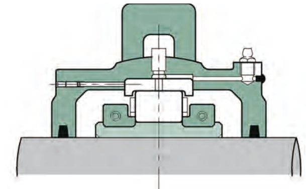
GR Bearing with Extra Axial Float
