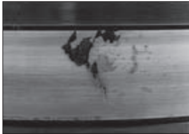
Point surface origin — Spalling from debris or raised metal exceeding the lubricant film thickness.
