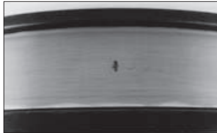
Inclusion origin — Spalling from oxides or other hard inclusions in bearing steel.
