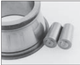
Abrasive wear — Fine abrasive particle contamination.
